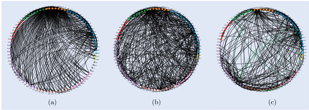
Figure 8. Network structure of the coefficient matrix constructed from forward-looking cross-impact models. (a) Based on best-level OFIs. (b) Based on integrated OFIs and (c) Based on returns.
