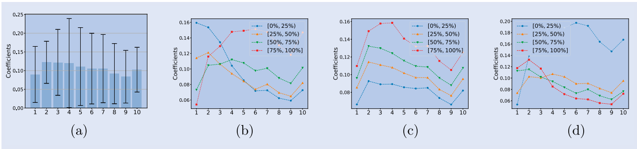
Figure A1. Coefficients of the model \mathbf{PI}^{[10]} . (a) Average. (b) Volume. (c) Volatility and (d) Spread. Note: Plot (a) reports average coefficients and one standard deviation (error bars); Plots (b)-(d) show coefficients sorted by stock characteristics. Volume: trading volume on the previous trading day. Volatility: volatility of one-minute returns during the previous trading day. Spread: average bid-ask spread during the previous trading day. [0%, 25%), respectively [75%, 100%], denote the subset of stocks with the lowest, respectively highest, 25% values for a given stock characteristic. The x -axis represents different levels of OFIs and the y -axis represents the coefficients.
