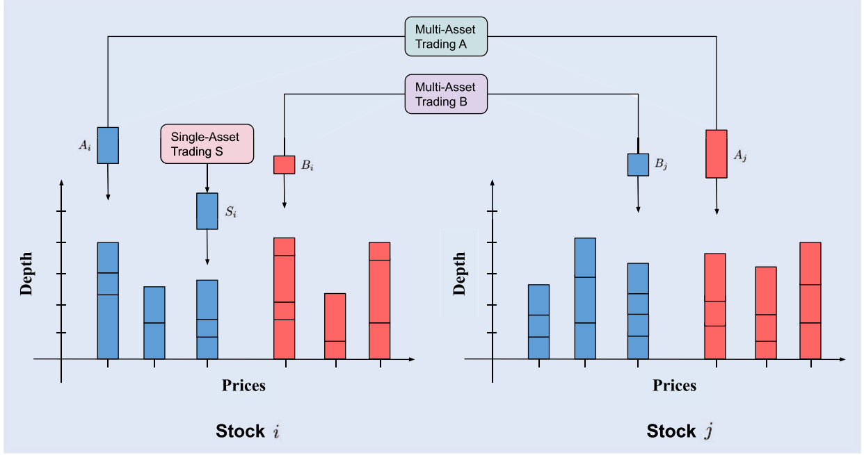
Figure 7. Illustration of the cross-impact model.
