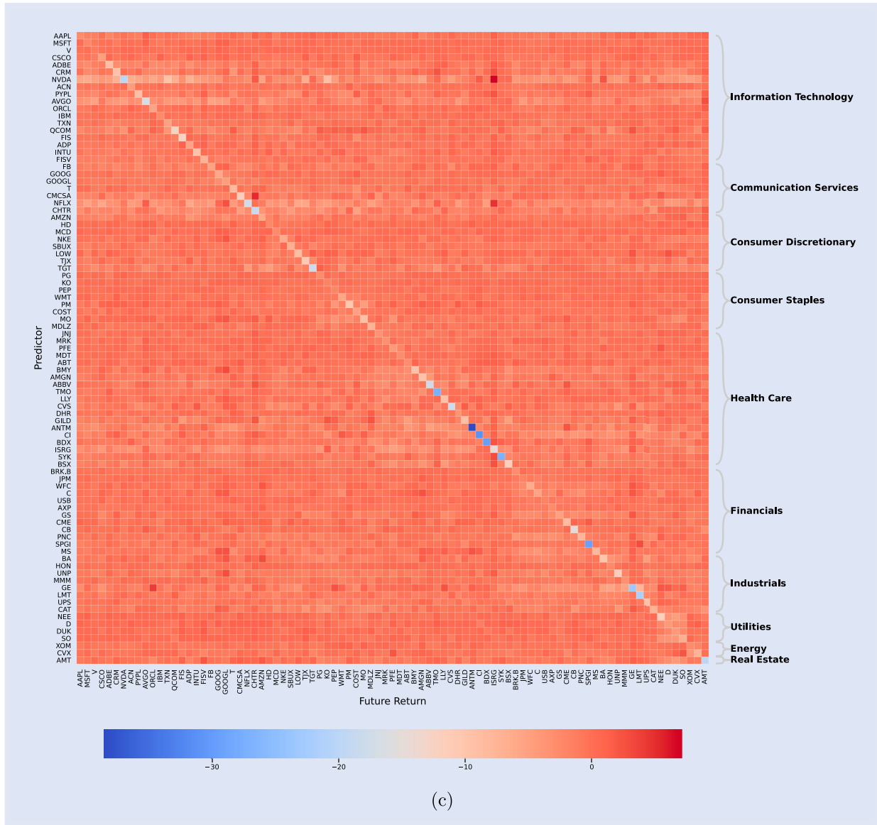
Figure A2. Continued. (c) Coefficient matrix of CAR .
