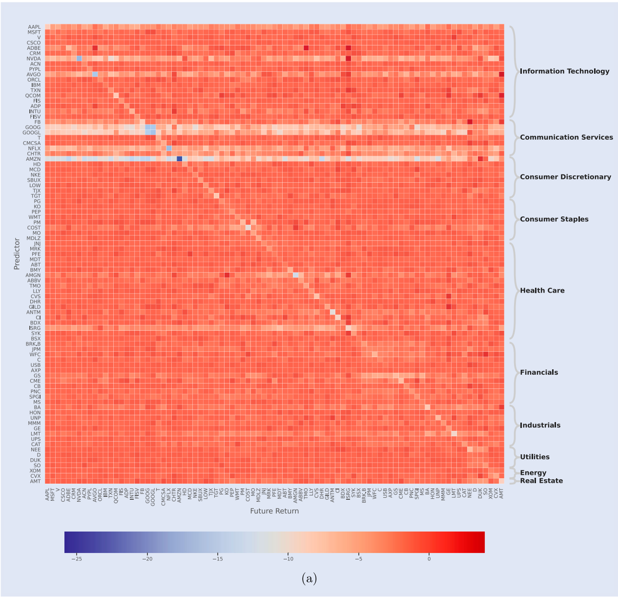
Figure A2. Average coefficient matrices constructed from forward-looking cross-impact models. (a) Coefficient matrix of \mathbf{FCI}^{[1]} .
