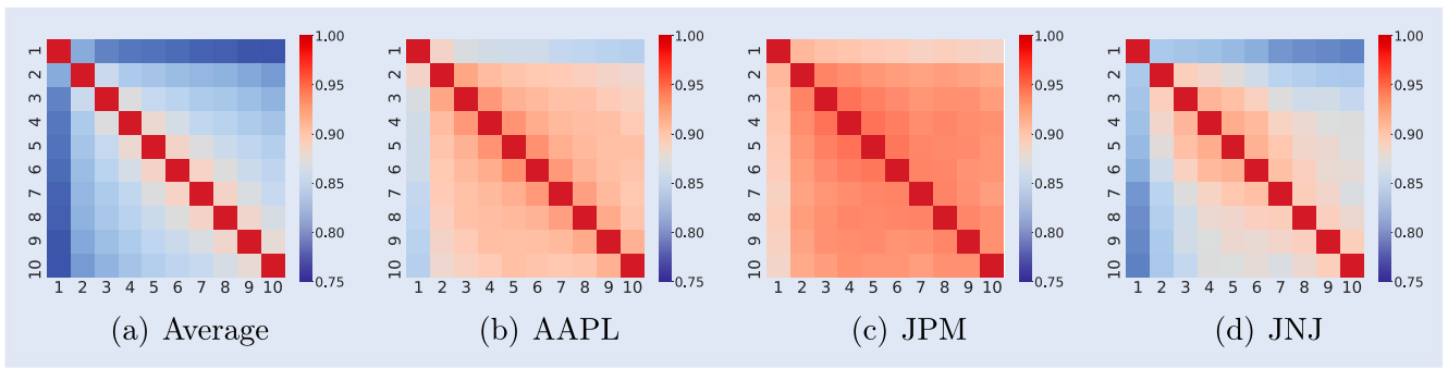
Figure 1. Correlation matrix of multi-level OFIs. (a) Average. (b) AAPL. (c) JPM and (d) JNJ.
