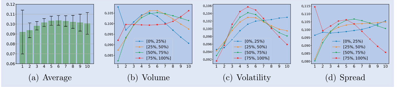
Figure 2. First principal component of multi-level OFIs, in quantile buckets for various stock characteristics. (a) Average. (b) Volume. (c) Volatility and (d) Spread.
