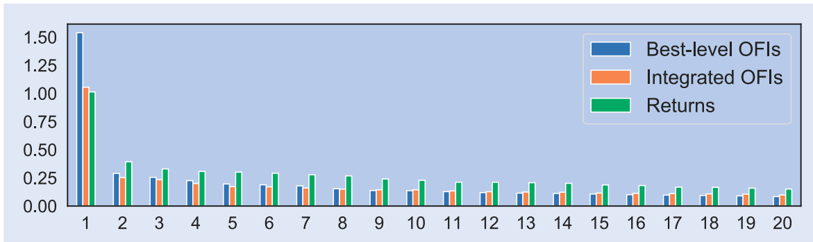
Figure 9. Barplot of normalized singular values for the average coefficient matrix in forward-looking cross-impact models.
