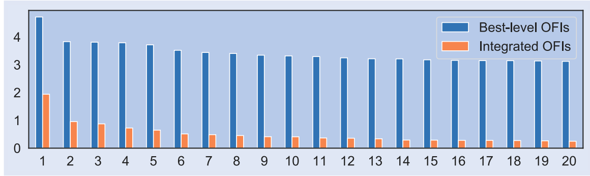
Figure 4. Barplot of singular values for the coefficient matrix in contemporaneous cross-impact models.
