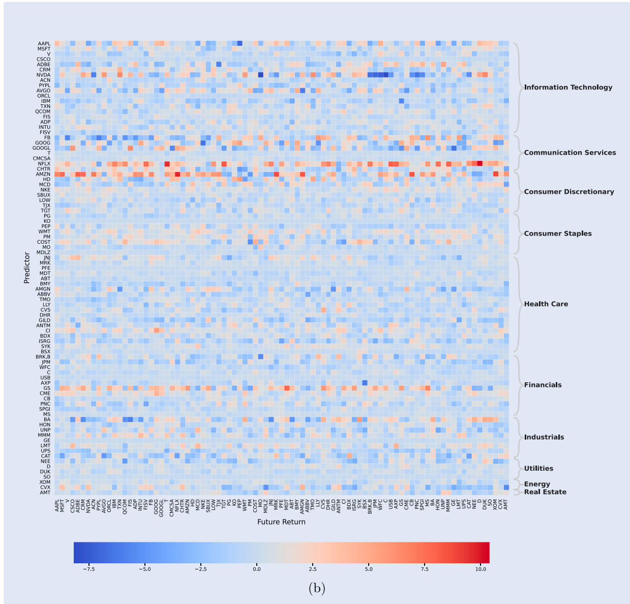
Figure A2. Continued. (b) Coefficient matrix of \text{FCI}^1
