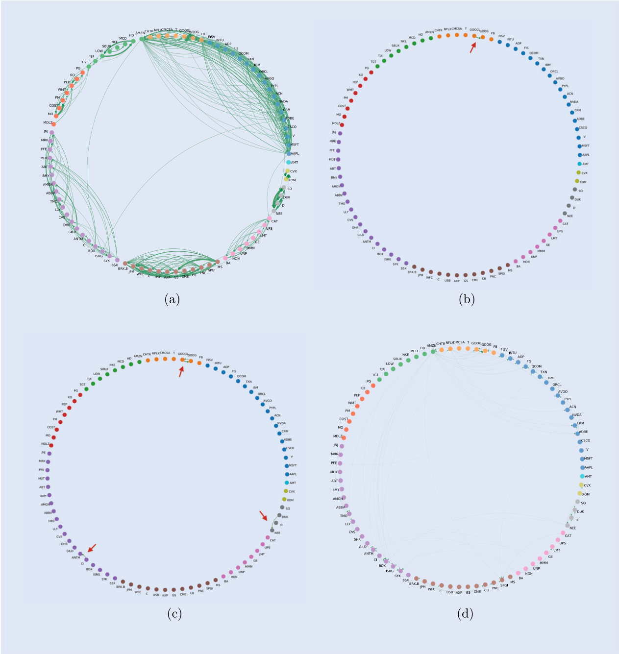
Figure 5. Illustrations of the coefficient networks constructed from contemporaneous cross-impact models. (a) Threshold = 95th percentile, based on best-level OFIs. (b) Threshold = 95th percentile, based on integrated OFIs. (c) Threshold = 75th percentile, based on integrated OFIs and (d) Threshold = 25th percentile, based on integrated OFIs. Note: To render the networks more interpretable and for ease of visualization, we only plot the top 5% largest (a-b), or top 25% largest (c), or top 75% largest (d), in magnitude coefficients. The coefficients are averaged over each regression window between 2017–2019. Nodes are colored by the GICS structure and sorted by market capitalization. Green links represent positive values while black links represent negative values. The width of edges is proportional to the absolute values of their respective coefficients.
