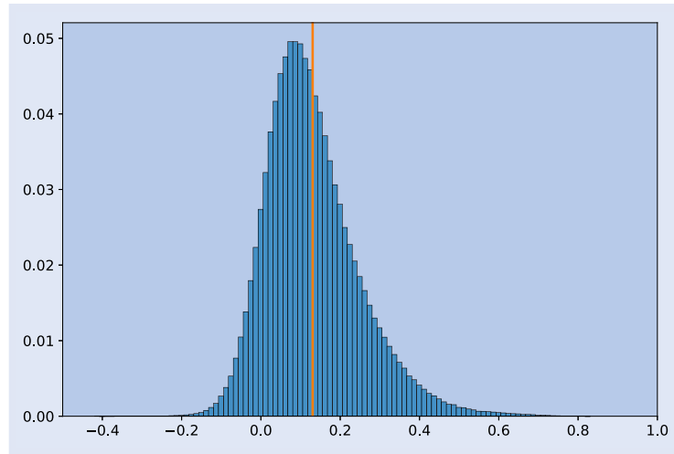
Figure 3. Distribution of correlations based on the best-level OFIs. Note: The orange vertical line represents the average correlation.
